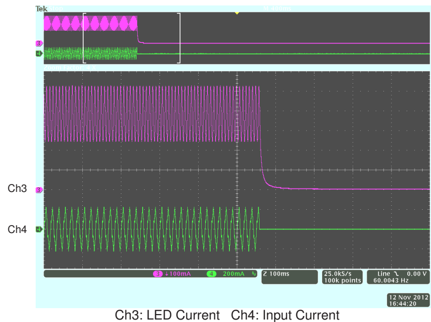
Figure 7. Enable Turn Off Waveform
