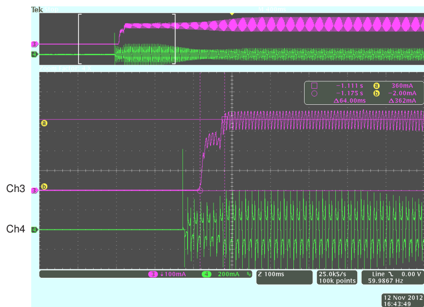
Figure 6. Enable Turn On Waveform – Turn On Time ~64 ms
