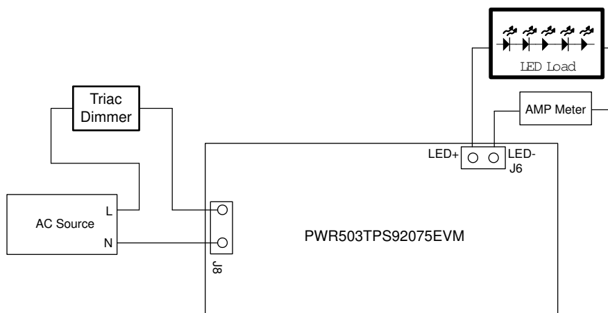
Figure 2. Dimming Wiring Diagram
