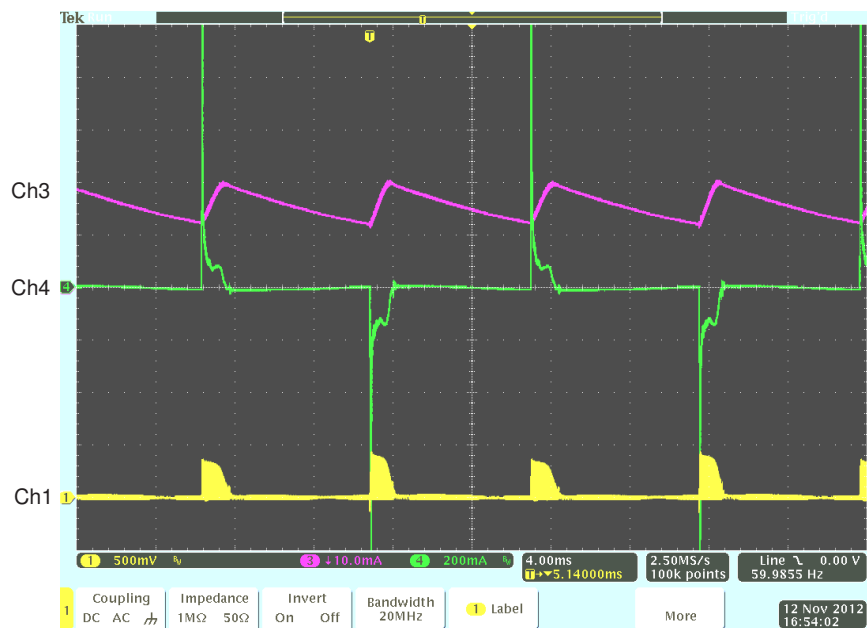
Figure 9. Leviton Leading Edge, Output = 20 mA
