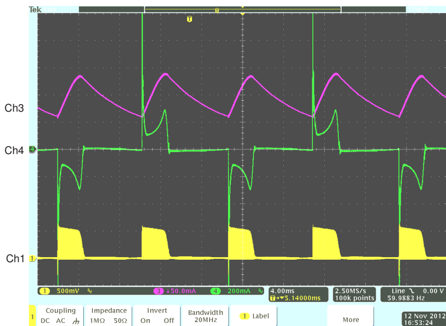
Figure 8. Lutron Leading Edge, Output = 100 mA
